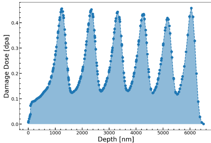
Figure 9: Combined damage dose plot for different thicknesses of an Al foil on a Cu layer under 3.25 MeV He irradiation. Fluence = 6.7e15 .
